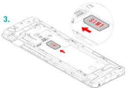
Micro SIM 1
